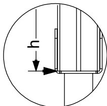
(R)-K1
