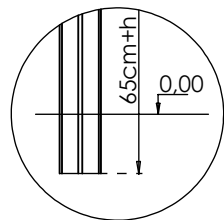
(R)-K1
