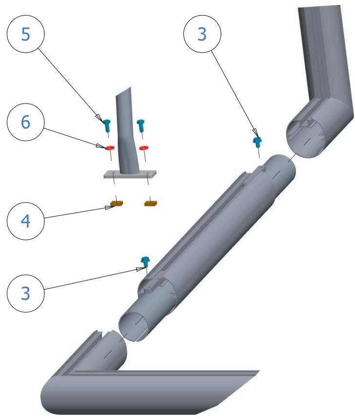
DETAIL B
